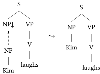
Figure 12.2: Substitution
