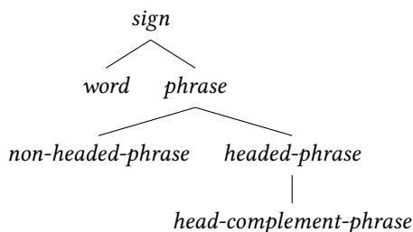
Figure 9.7: Type hierarchy for sign : all subtypes of headed-phrase inherit constraints
