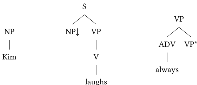
Figure 12.1: Elementary trees
