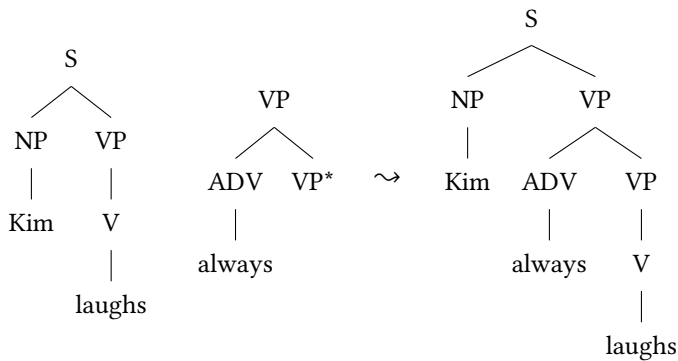
Figure 12.3: Adjunction
