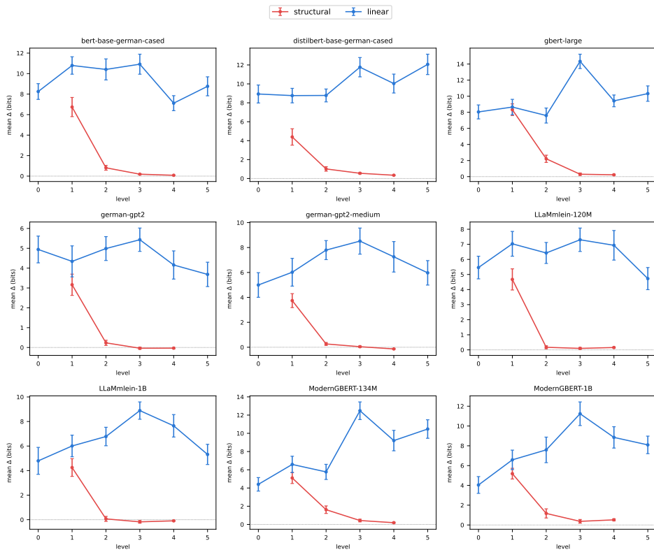
Figure 24.1: The delta of the surprisal values with dative and accusative for various LLMs
