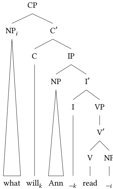
Figure 3.7: wh -question
