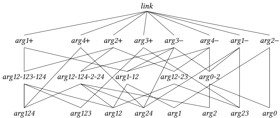
Figure 21.4: Hierarchy of argument frames following Haugereid (2007)
